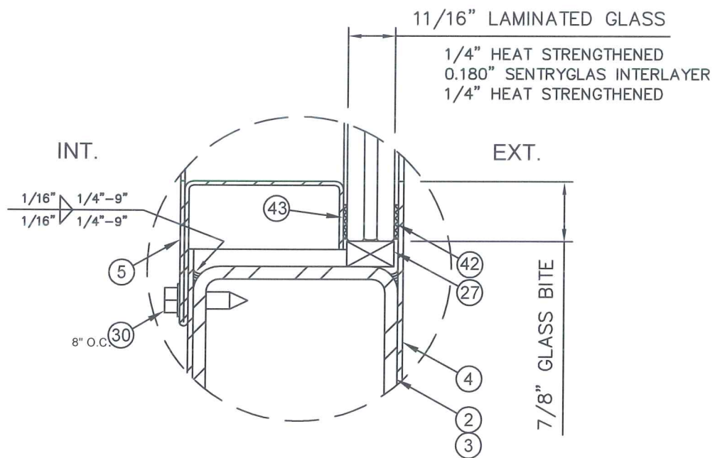
INSIDE GLAZED
