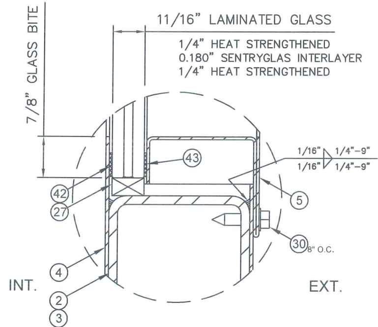
OUTSIDE GLAZED
